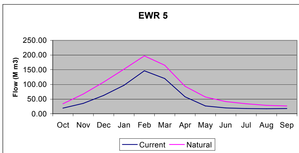
Figure A34 Flow duration curve for EWR 5
